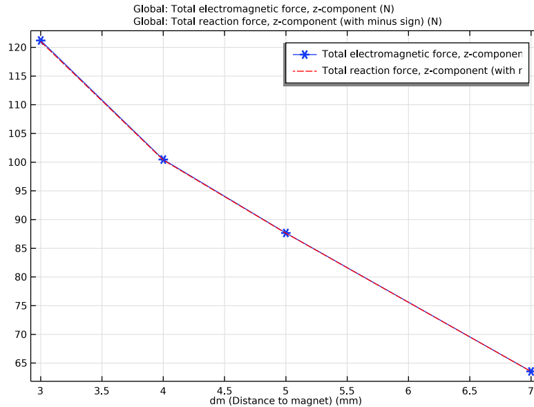
Figure 9: The total pulling magnetic force and the total structural reaction force (re-computed for the full geometry).
