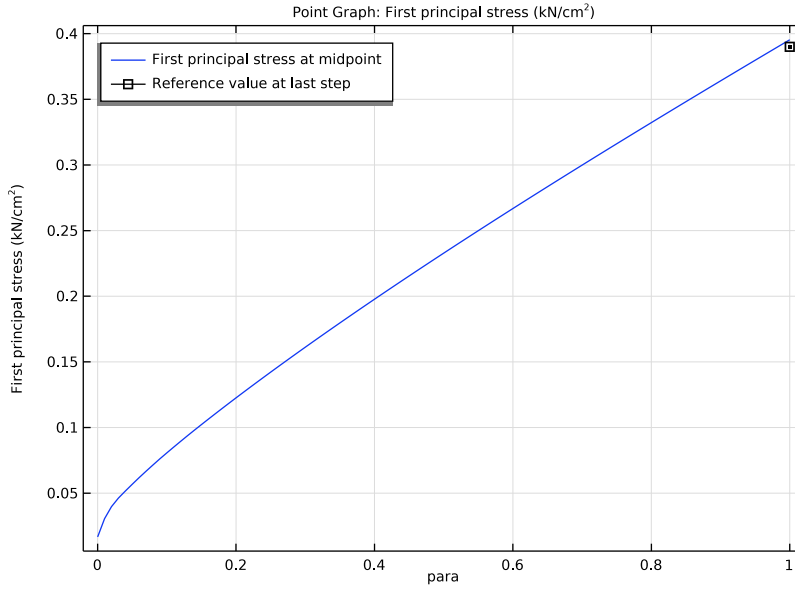
Figure 6: First principal stress at midpoint.
