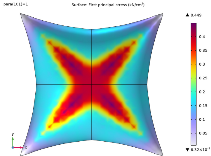
Figure 3: First principal stress after inflation.
