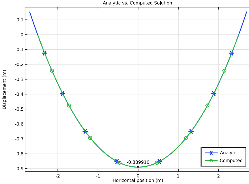
Figure 3: Cable sag due to self-weight (load case 1). Comparison of the analytical and the solution computed using the Wire interface.
