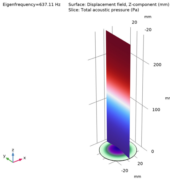
Figure 5: Disc deformation and pressure contours for the first coupled mode.
