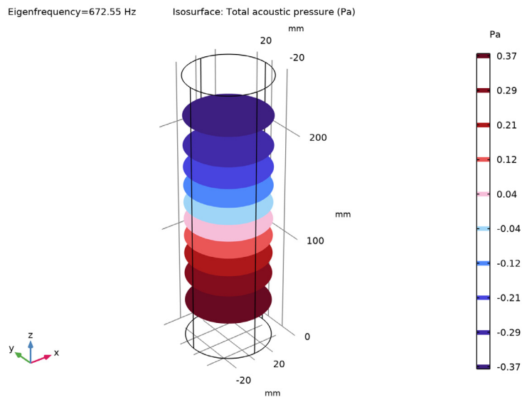
Figure 3: First acoustic mode displayed by pressure isosurfaces.
