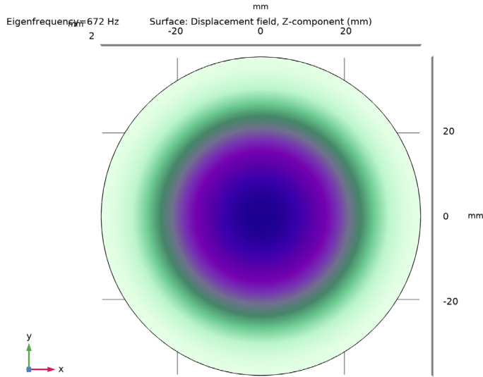
Figure 1: First structural mode displayed by vertical displacement.
