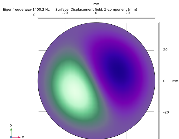
Figure 2: Second structural mode displayed by vertical displacement.
