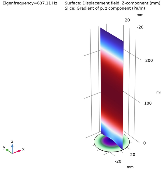
Figure 6: Disc deformation and pressure gradient contours for the first coupled mode.
