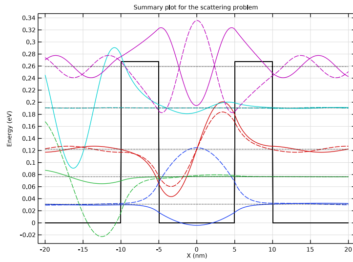
Figure 4: Stationary study solutions of five selected energies.
