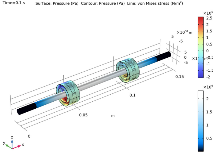
Figure 2: Pressure and stress in the turbocharger.
