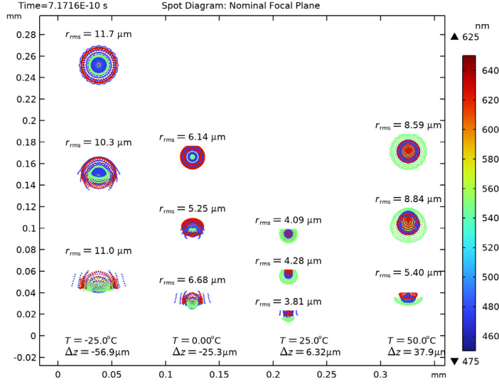
Figure 10: The image quality on the nominal image plane as a function of temperature. This plane is coincident with the detector surface after deformation. \Delta z = z(T) - z(T=20^\circ\text{C}) .
