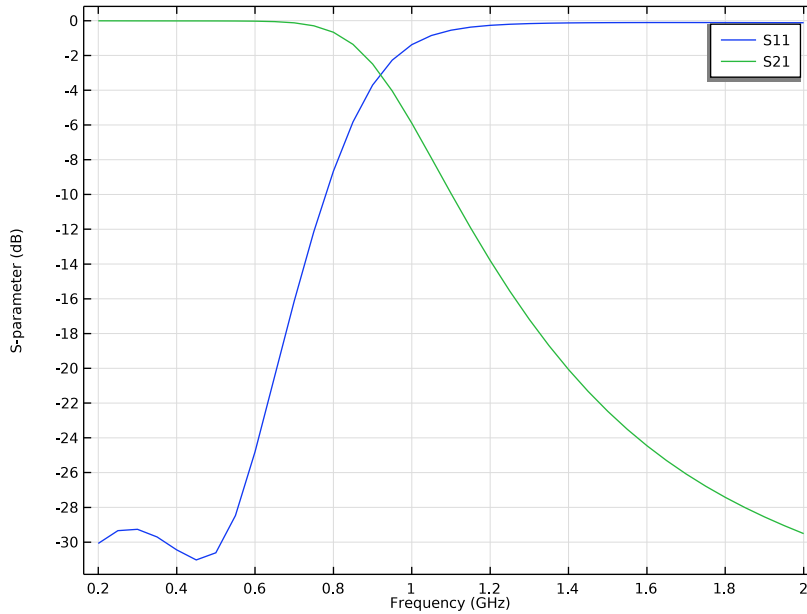
Figure 3: S-parameter plot shows the frequency responses of a low-pass filter.
