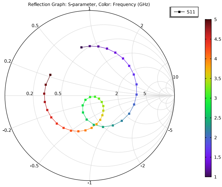
Smith Plot (emw)
