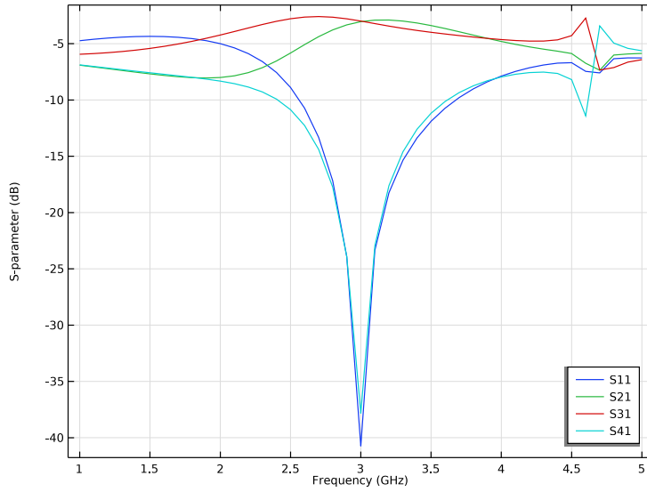
Figure 3: The frequency response of the branch line coupler shows good input matching ( S_{11} ) and isolation ( S_{41} ) around 3 GHz. The coupled signal at the two output ports ( S_{21} and S_{31} ) is about -3 dB at 3 GHz.
