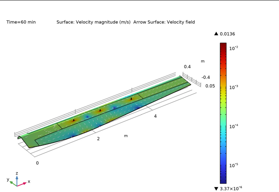
Figure 2: Velocity magnitude in logarithmic scale plotted on a cross section in the middle of the mold.
