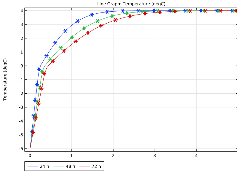
Figure 1: Computed (solid line) compared to analytical solution (asterisks) after 24, 48, and 72 h.
