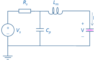
Figure 2: L-match used in this model.
