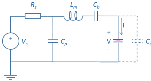
Figure 1: L-match including blocking and stray capacitance.
