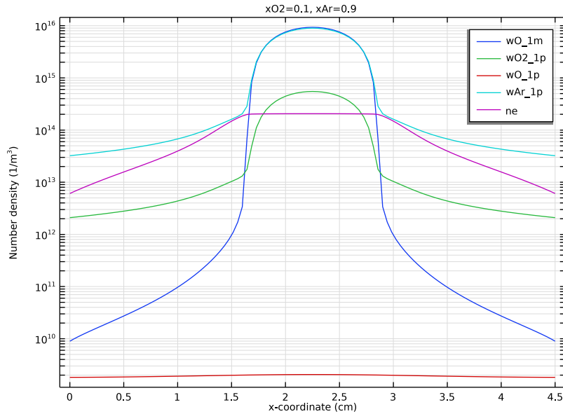
Figure 2: Spatial distribution of period averaged number densities of charged species for a O_2 mole fraction of 0.1.
