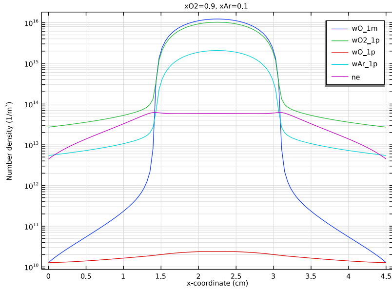
Figure 1: Spatial distribution of period averaged number densities of charged species for a O_2 mole fraction of 0.9.
