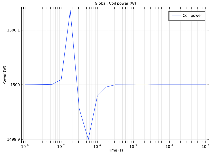
Figure 6: Plot of total power vs. time in GEC ICP reactor.
