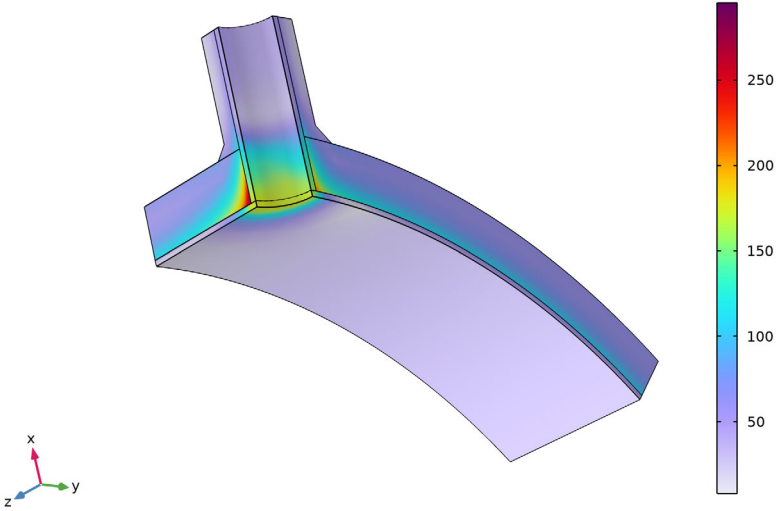
Figure 4: Distribution of von Mises stress after cooling down the hot water.
