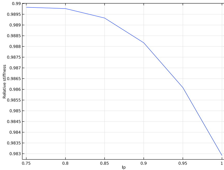
Figure 6: The normalized cut reaction force as function of the load multiplier.
