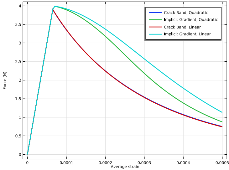
Figure 3: Force versus prescribed end displacement.
