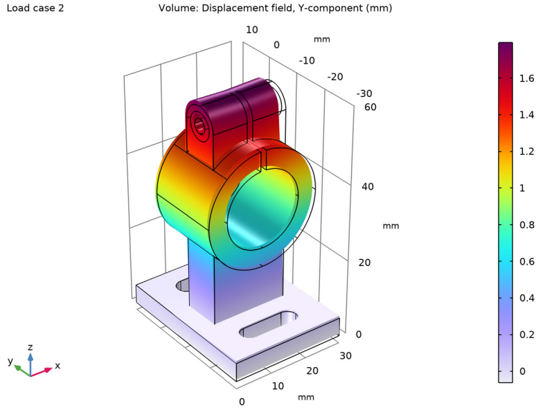
Figure 3: Displacement of the clamp in the loading direction in case of only one mounting bolt.
