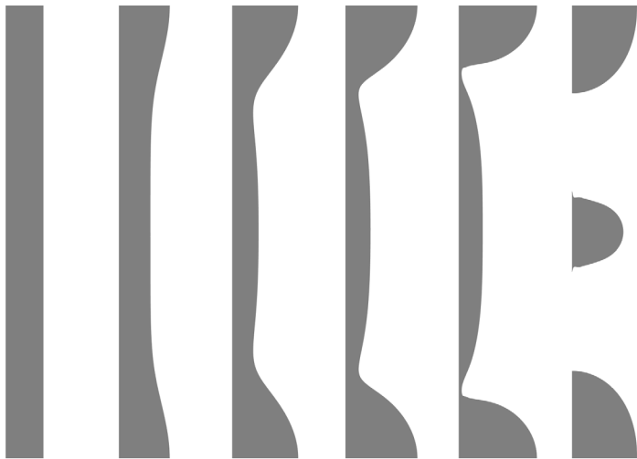
Figure 2: Liquid regions of the model (black), obtained from the level set method, shown at 6 different times: 0, 6, 9, 10, 11, and 16.4\mu\text{s} .
