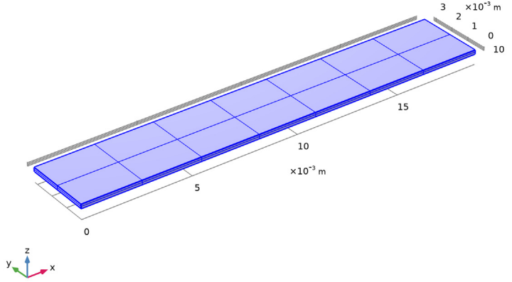
Figure 2: Model mesh.
