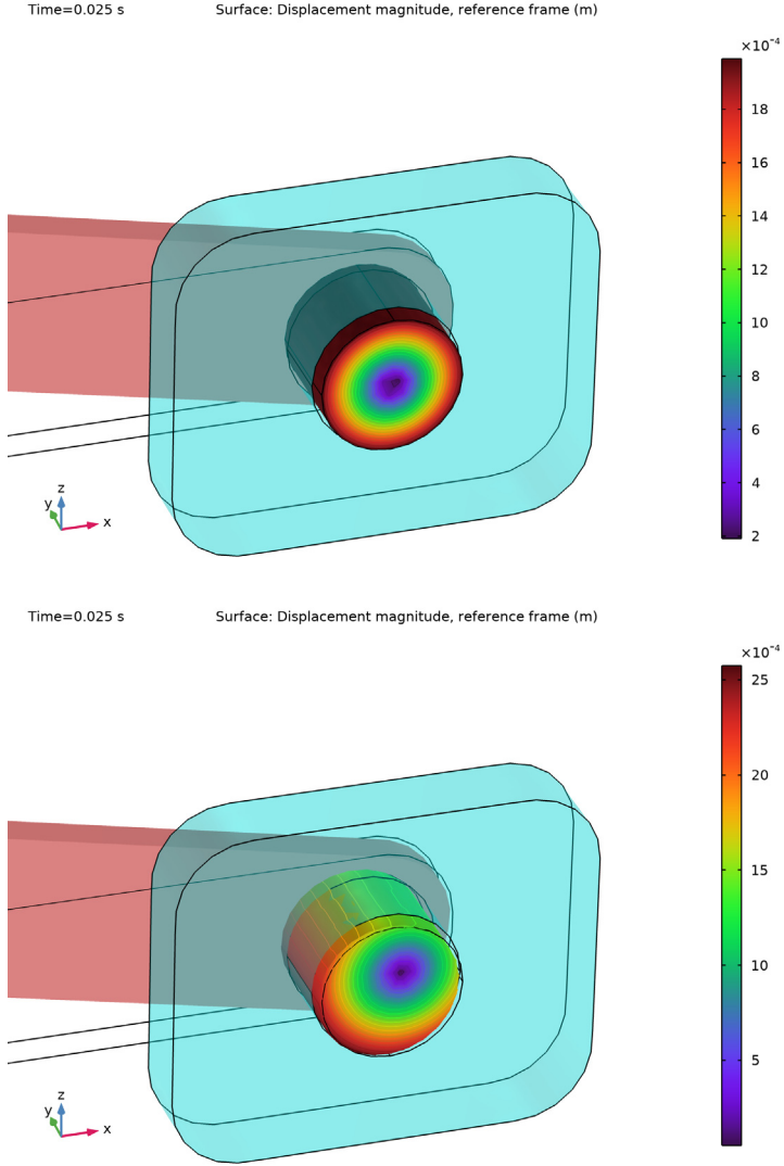
Figure 3: Relative displacement of connecting rod journal with respect to the slider for hinge joint and clearance joint cases respectively at t = 0.025 s.
