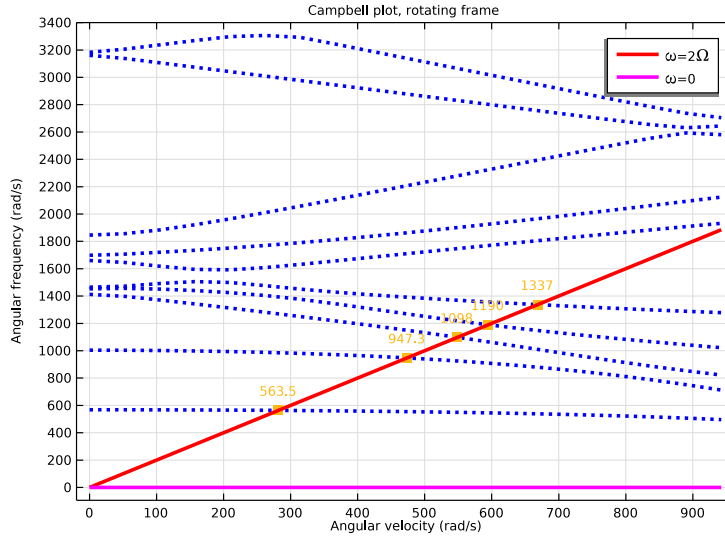
Figure 3: Campbell diagram.
