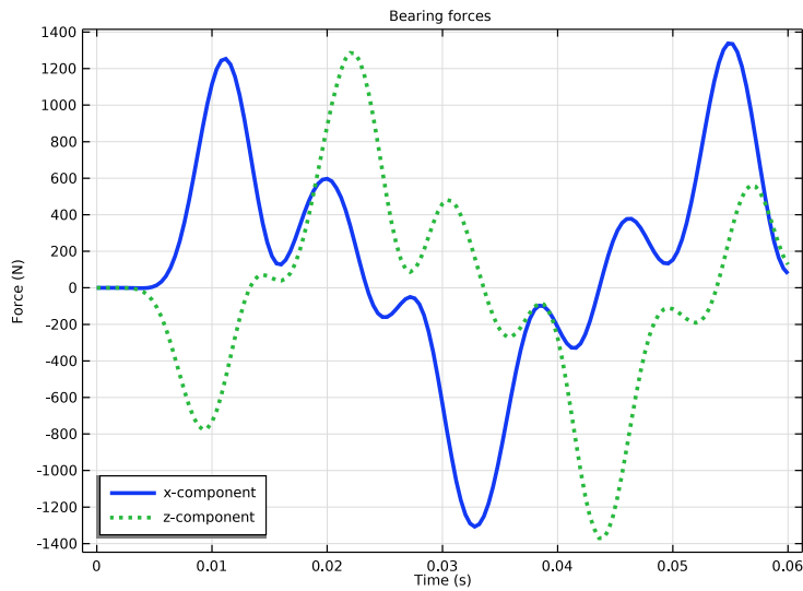
Figure 10: Time variation of the bearing forces.
