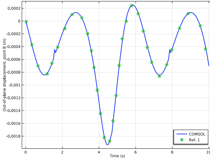
Figure 3: Comparison of out-of-plane displacement of point B with Ref. 1.
