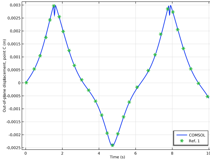
Figure 4: Comparison of out-of-plane displacement of point C with Ref. 1.
