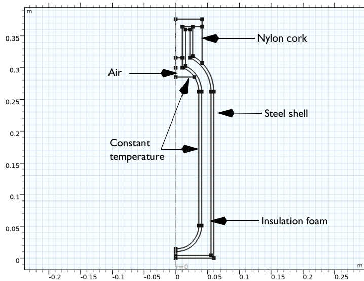
Figure 1: Cross section of the vacuum flask geometry.
