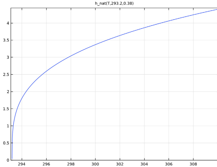
Figure 3: Heat transfer coefficient for natural convection cooling of a vertical wall versus the surface temperature. The ambient temperature and the wall length are given constant, T_{\text{ambient}} = 293.2 \text{ K} and L = 38 \text{ cm} , respectively.
