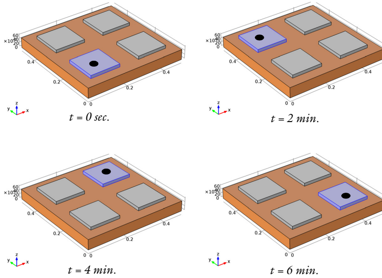
Figure 1: Model geometry with the copper plate in orange and the active steel plate in blue marked by a filled circle.
