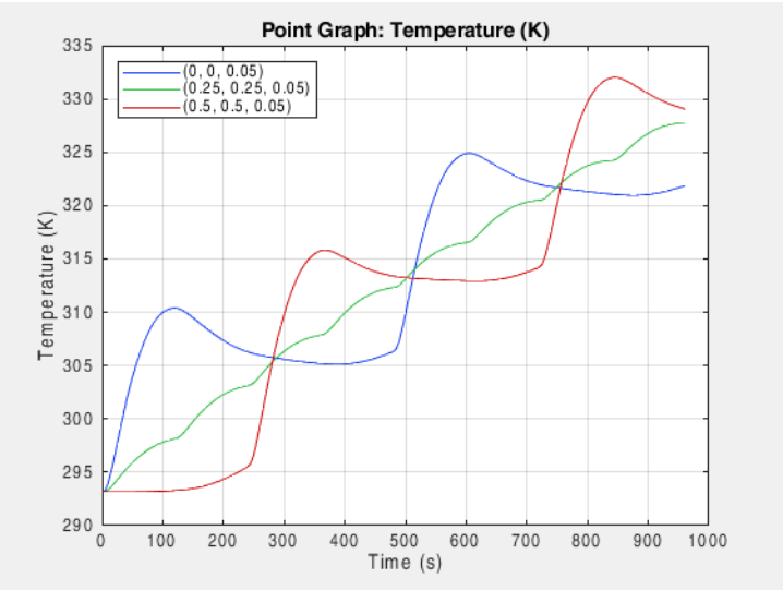
Figure 2: The temperature at two of the corners and in the middle of the top surface of the copper plate.
