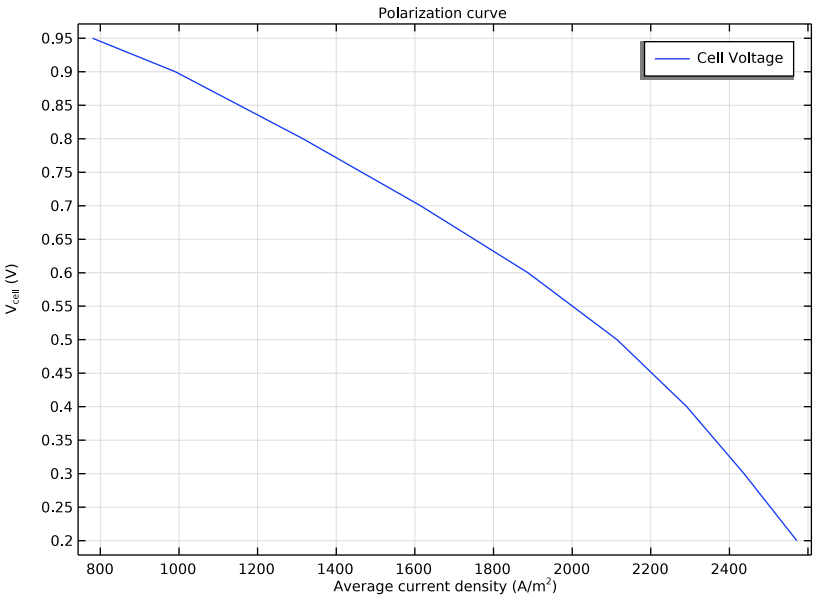
Figure 5: Polarization curve.
