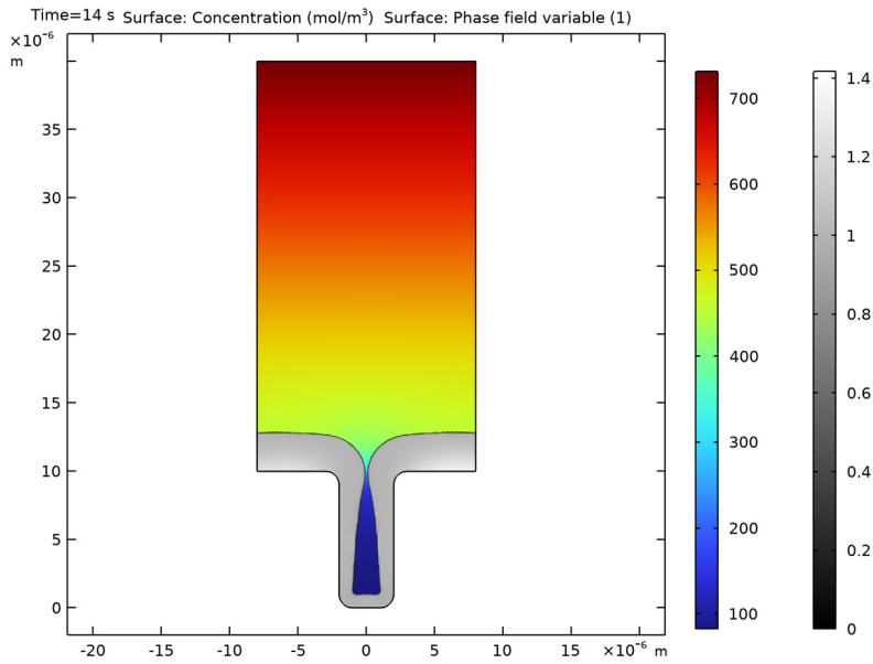
Figure 4: Surface plot of concentration of copper ions along with the phase field variable contour of value 0.5 after 14 seconds of deposition operation using the Phase Field interface.
