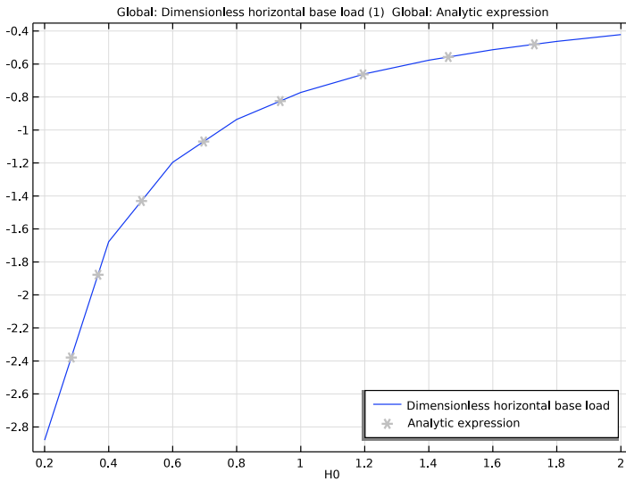
Figure 7: Nondimensional horizontal base load vs film thickness ratio, H_0=h_0/s_h . The computed results are shown as the continuous curve and the theoretical result as the gray symbols.
