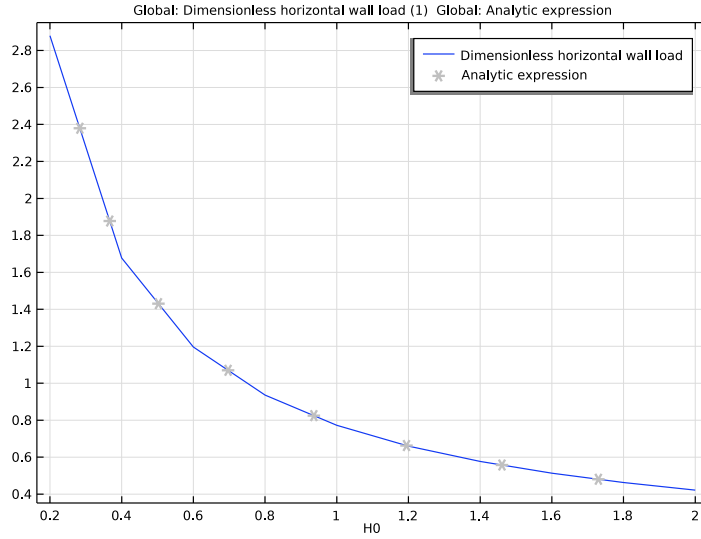
Figure 6: Nondimensional horizontal wall load vs film thickness ratio, H_0=h_0/s_h . The computed results are shown as the continuous curve and the theoretical result as the gray symbols.
