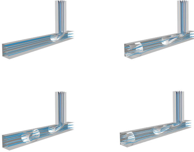
Figure 3: Velocity streamlines and the phase boundary at t = 0.02\text{ s} , 0.04\text{ s} , 0.06\text{ s} , and 0.08\text{ s} .
