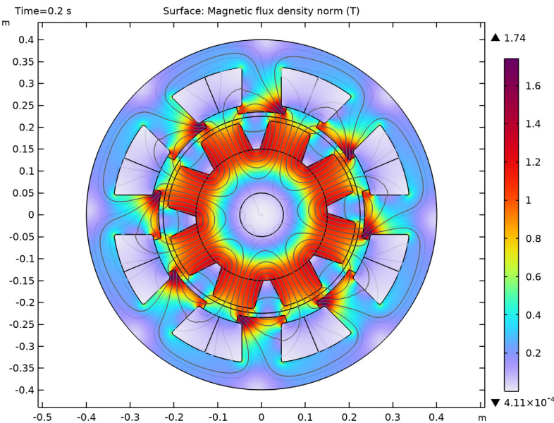
Figure 4: The norm and the field lines of the magnetic flux density after 0.2 s of rotation. Note the darker regions, which indicate the position of the permanent magnets in the rotor.
